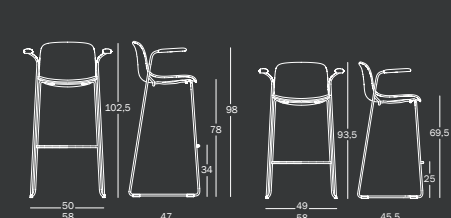
Troy stool, sledge / front seat covered w/ arms
