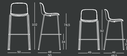
Troy stool, 4 legs / front seat covered
