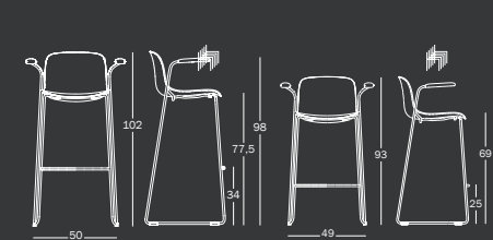
Troy stool, sledge / polypropylene w/arms
