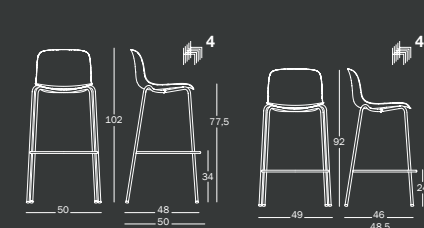
Troy stool, 4 legs / front seat covered
