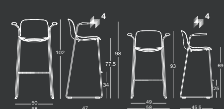
Troy stool, sledge / fully covered w/arms
