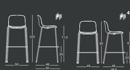
Troy stool, 4 legs / fully covered
