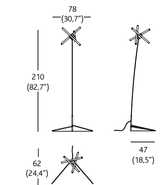
Standing lamp / De pie
